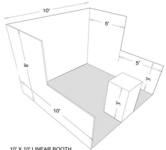
10' X 10' LINEAR BOOTH
