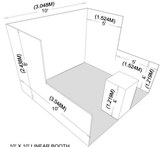
10' X 10' LINEAR BOOTH
